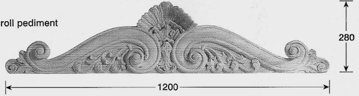
CAPE30LW Large palmette scroll pediment Max depth 60 Base thickness 25
