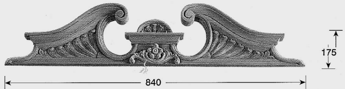
CAPE4 Roman pediment Base thickness 15
